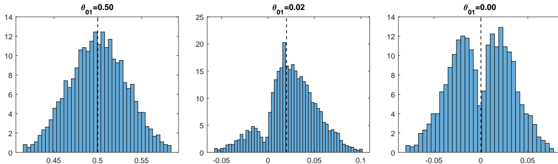
Figure 4: Linear Gaussian MLE
